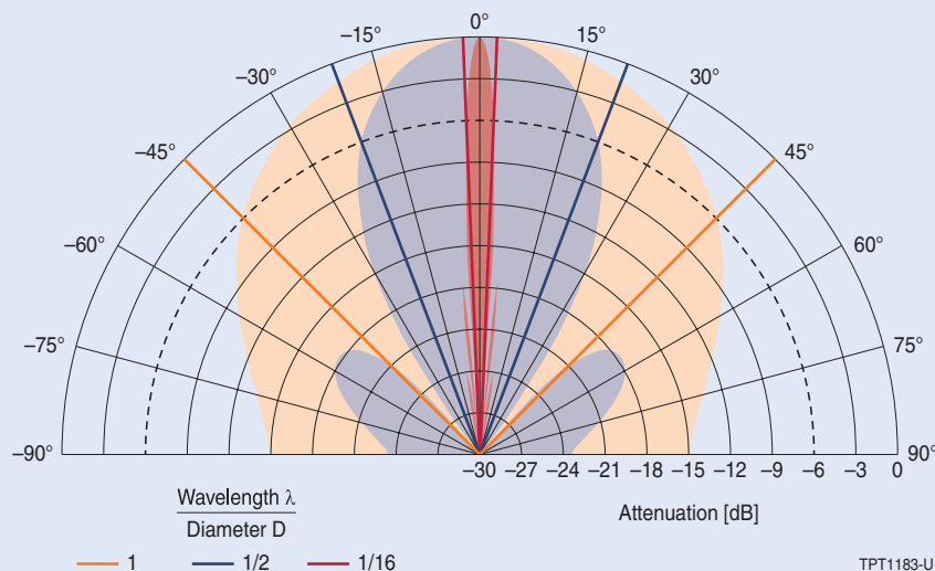
Directivity of sound pressure level calculated for various membrane geometries (unclamped).
