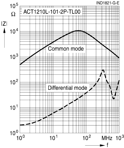
Impedance versus frequency (typical values) ACT1210L-101-2P-TL00
